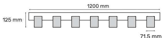
HarmonyGrid_120 A-F / HarmonyGrid_120 B-F 1200 x 1200 x 125 mm
