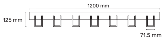
HarmonyGrid_120 A / HarmonyGrid_120 B 1200 x 1200 x 125 mm
