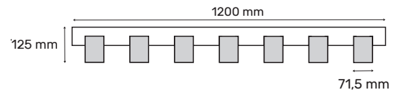
HarmonyGrid_120 A-F / HarmonyGrid_120 B-F 1200 x 1200 x 125 mm
